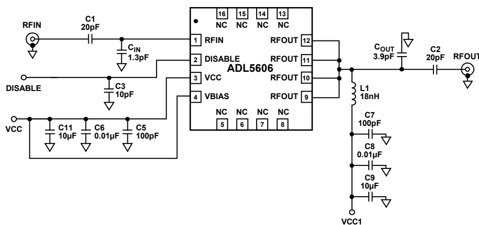
Figure 31. Basic Connections
